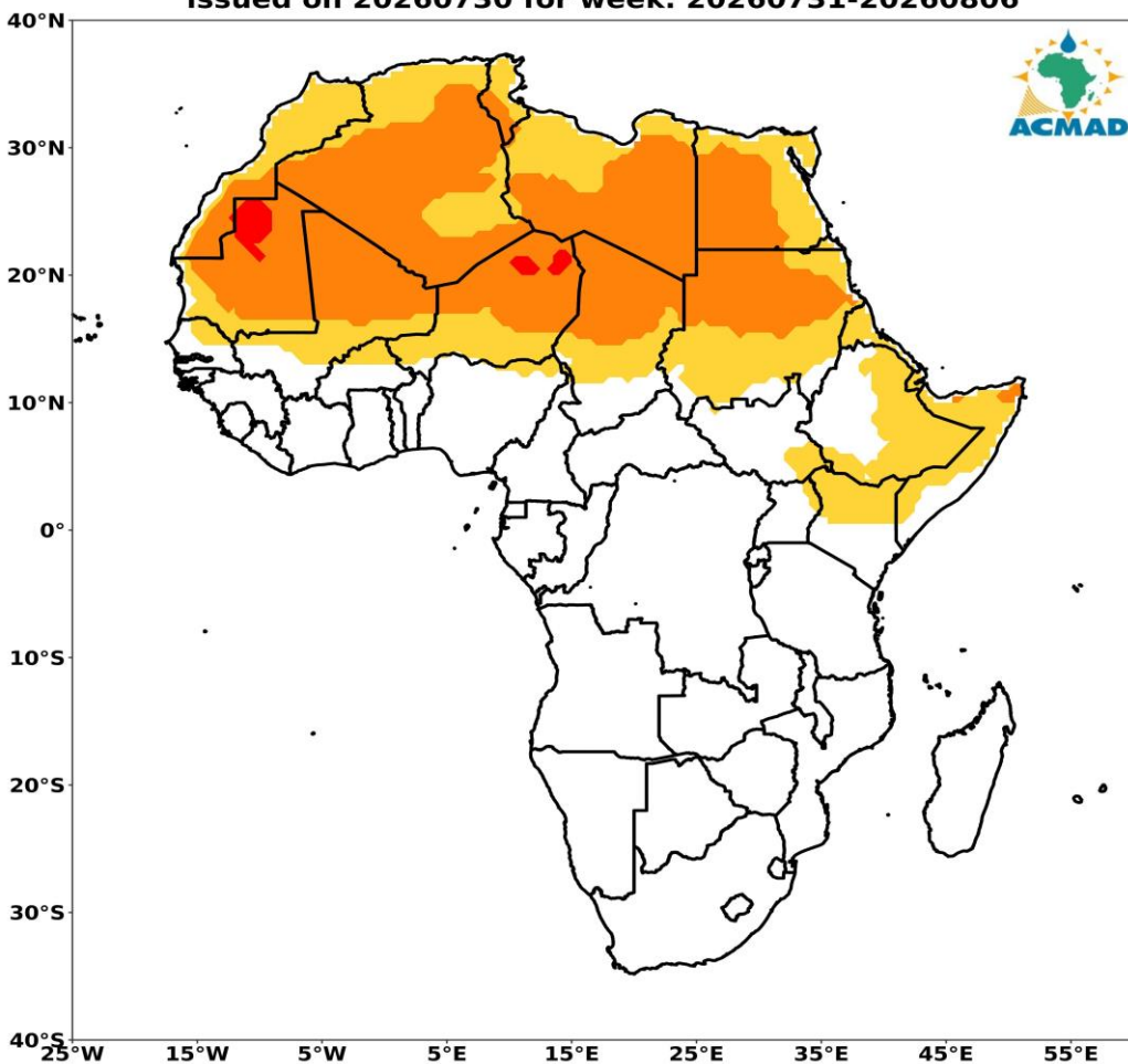
VIGILANCE MAP FOR MENINGITIS OUTBREAKS IN AFRICA issued on 20260730 for week: 20260731-20260806
